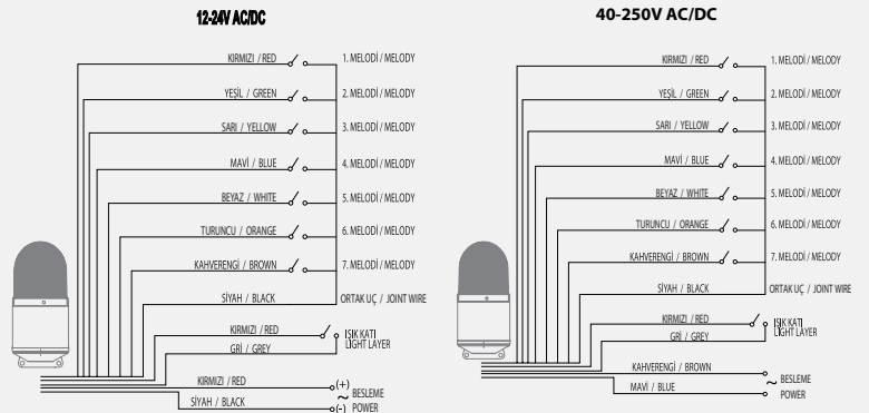
SNT-EK7013-F1-4
