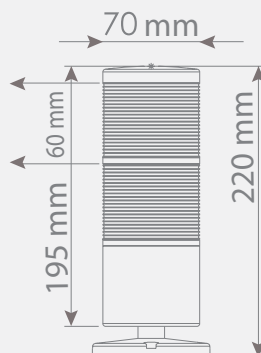
SNT-7013-F2-D-20U
