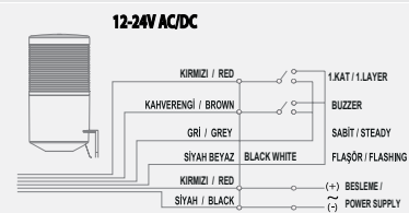
SNT-K7013-F1-4
