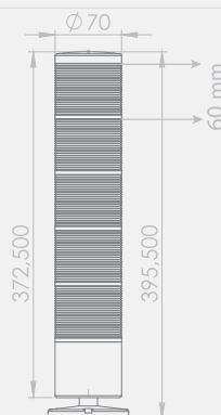
SNT-7013-F5-D-20U
